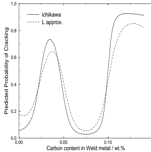
Figure 8. Carbon Dependence of Weld Cracking probability: These graphs show the predictions as a function of one of the 13 input variables given by a committee of neural networks (Ichikawa et al. 1996) and those found using the lower bound approximation of a VGC. Both have the same large scale features.
