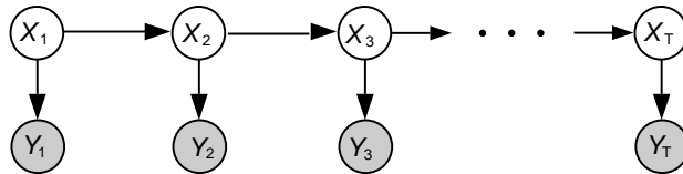
Figure 3 Bayesian network representation of a state-space model.
